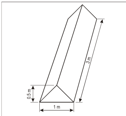
Figure 5-34. Boundary marker
