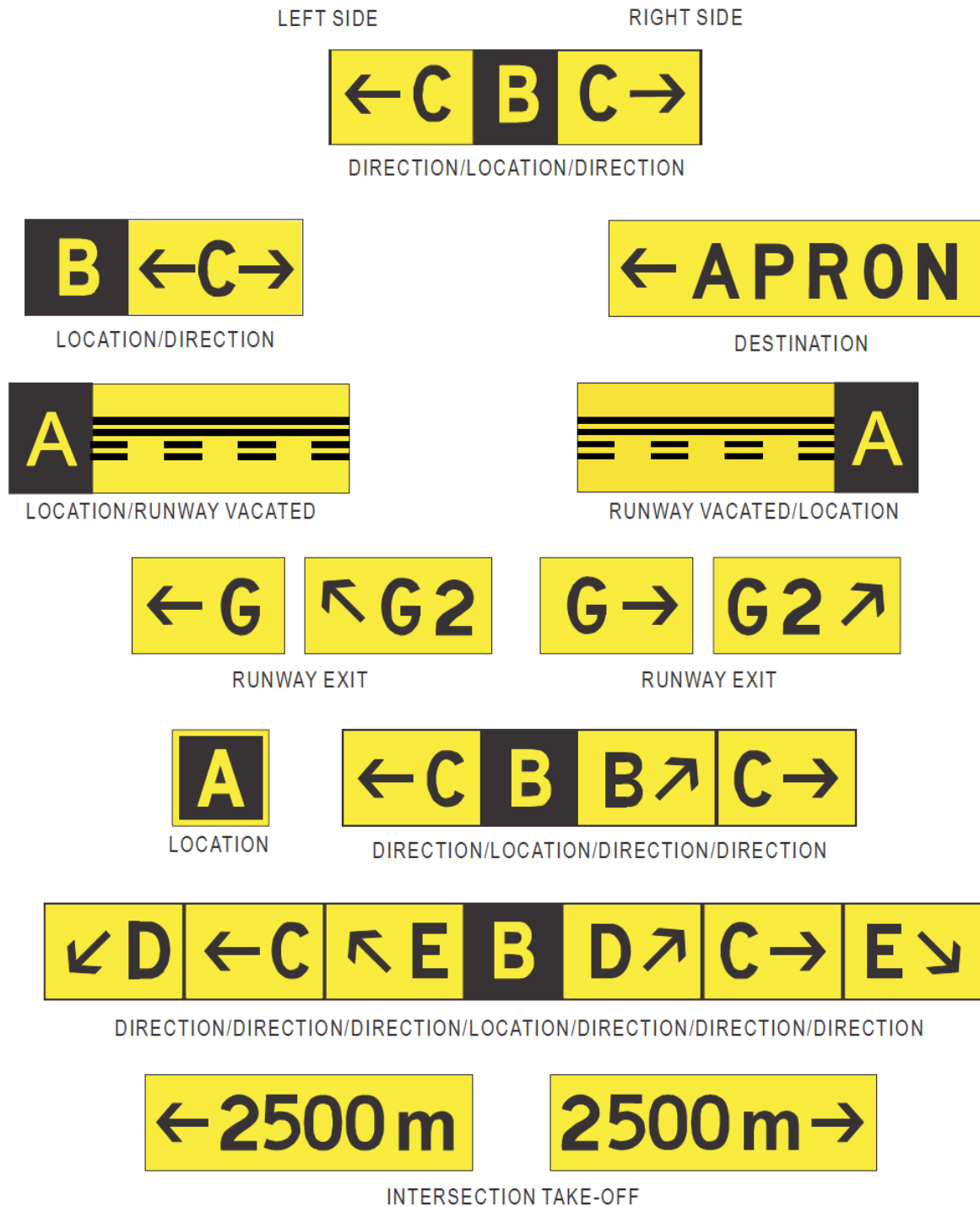
Figure 5-31. Information signs
