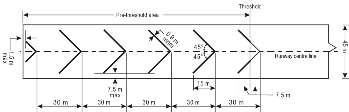
Figure 7-2. Pre-threshold marking
