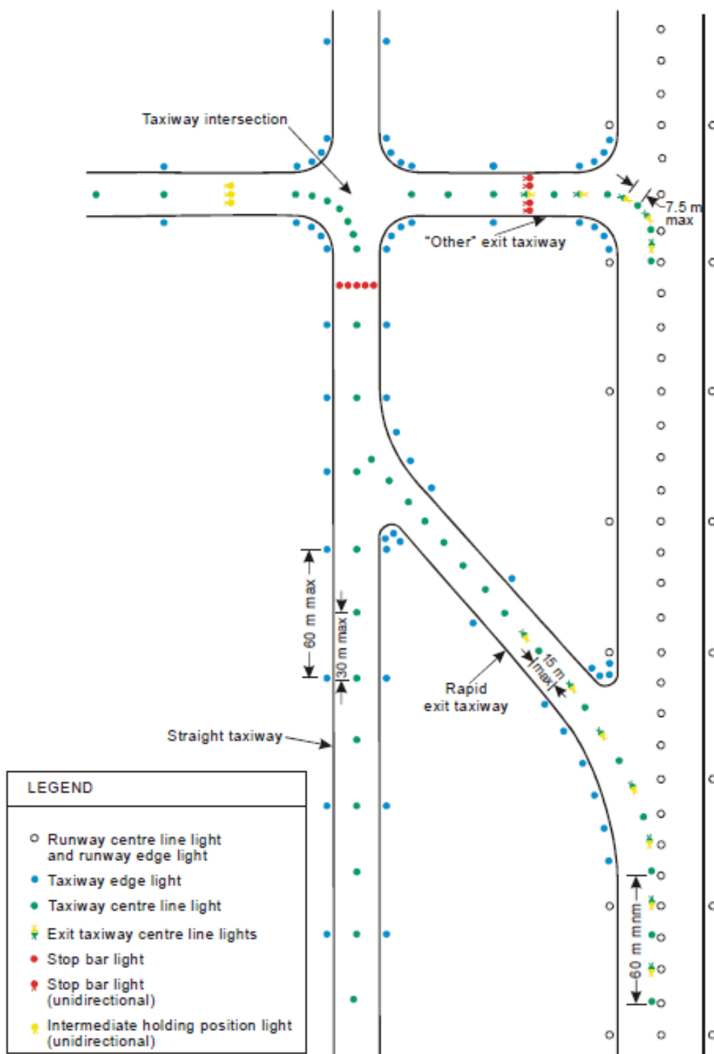
Figure 5-26. Taxiway lighting
