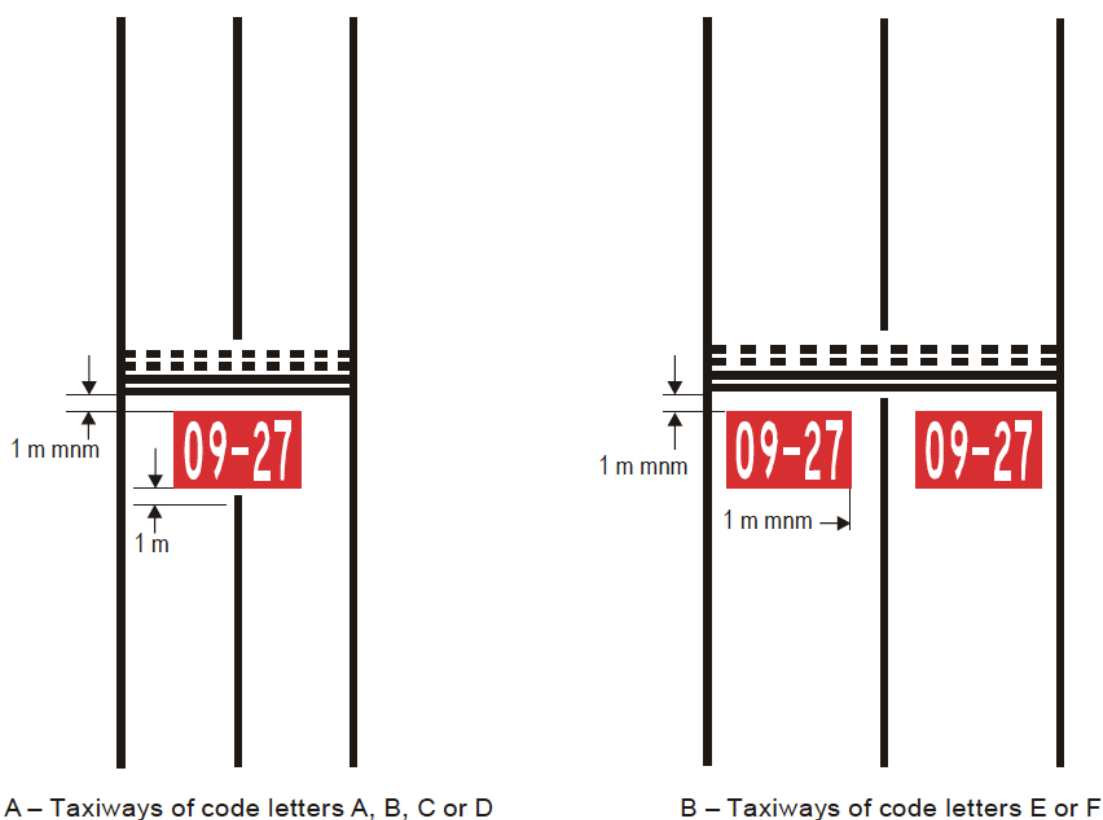
Figure 5-10. Mandatory instruction marking
