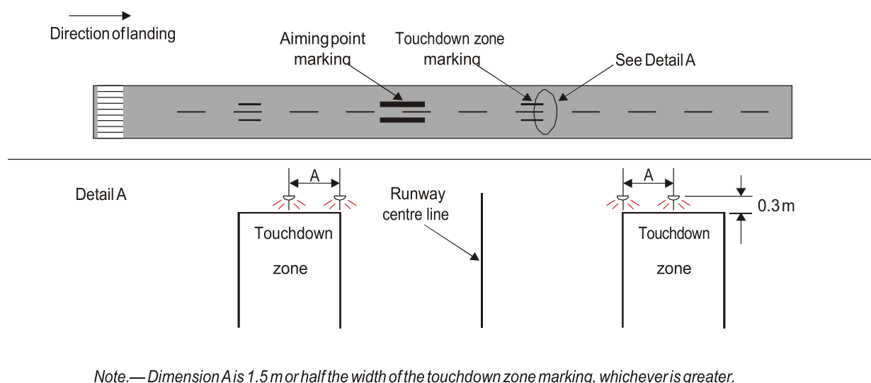
Figure 5-24. Simple touchdown zone lighting
